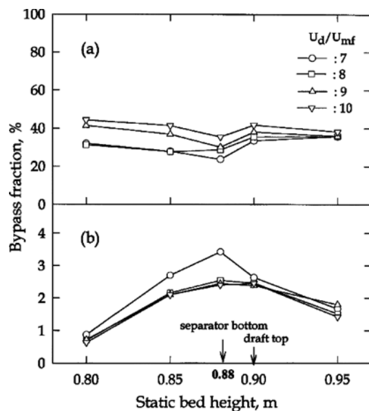
Fig. 3. Effect of static bed height on the gas bypass fraction with different U_a .
