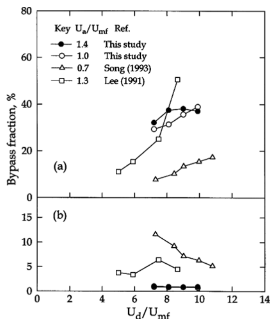
Fig. 6. Effect of U_d on the gas bypass fraction.
