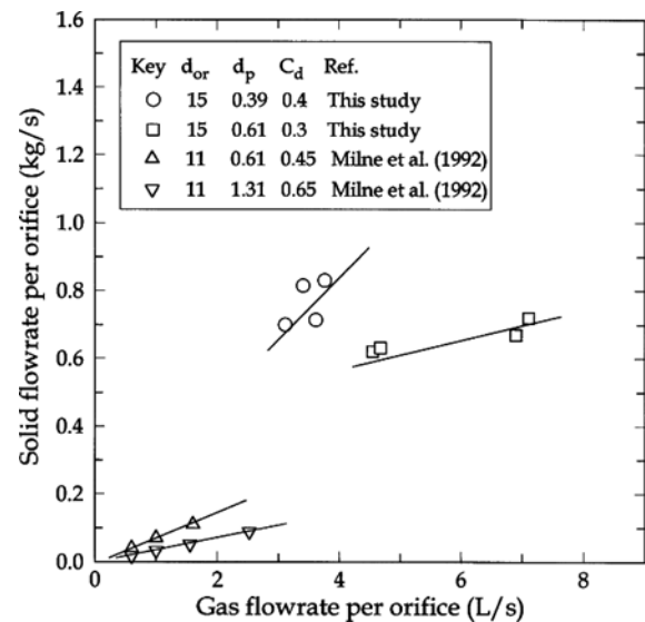
Fig. 10. Comparison of gas flow rate and solids flow rate through the orifice.
