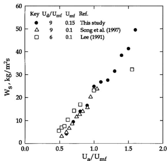
Fig. 4. Effect of U_a on W_s .
